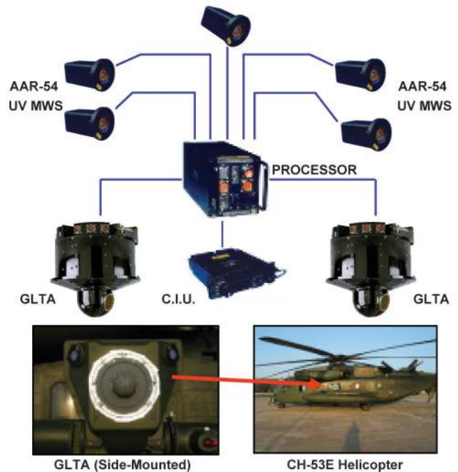
GLTA (Side-Mounted) CH-53E Helicopter C.I.U. - Control Interface Unit GLTA - Guardian Laser Turret Assembly MWS - Missile Warning System UV - Ultraviolet
